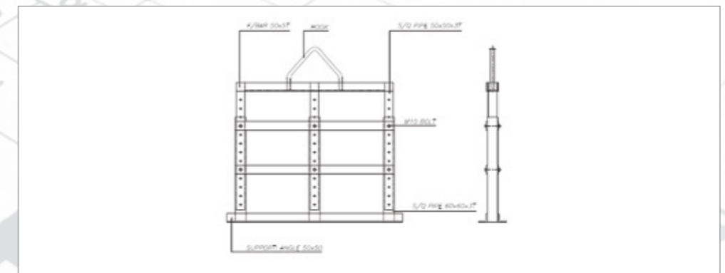
A HEIGHT ADJUSTABLE HANGER TYPE CAGE
