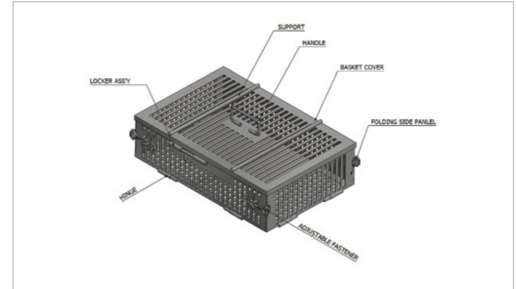
REMOVABLE CASE FOR CHARGING FISHING & FREEZING THE SAME
